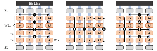
(a) Horizontal-first order. (b) Vertical-first order. (c) Mixed order. Figure 12: Examples of different program orders in 3D flash.
