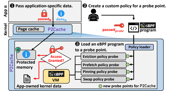
Figure 3: An operational overview of P2Cache.
