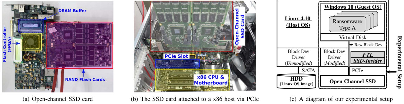
Fig. 6: SSD-Insider's working prototype and experimental setup
