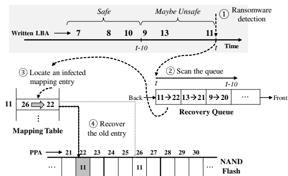
Fig. 5: Data recovery process in SSD-Insider. After ransomware is detected (①) at time t , the SSD-Insider FTL scans the recovery queue (②), examining LBAs, old PBAs, and timestamps. For LBAs 9, 13, and 11 that were recently overwritten (i.e., > t - 10 ), the SSD-Insider cannot guarantee their safety. Therefore, SSD-Insider locates a mapping entry in the mapping table (③) and updates the entry so that it points to the physical location of the original data (④). In case of LBA 11, its mapping entry is reverted from PPA 26 to PPA 22 that contains old but safe data. For LBAs 7, 8, and 10 that were written 10 seconds ago (i.e., \leq t - 10 ), SSD-Insider guarantees that their data are safe, and thus their mapping entries are not updated.
