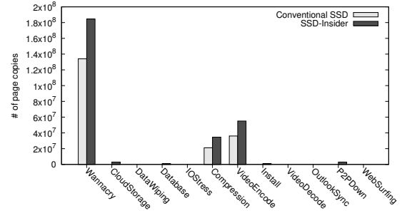
Fig. 9: A comparison of GC costs
