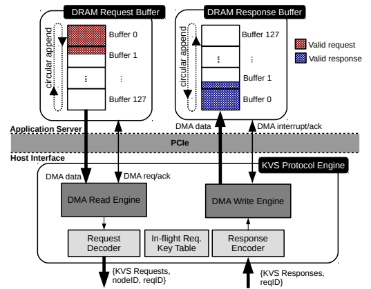
Figure 6: Application to KVS Protocol Engine communication
