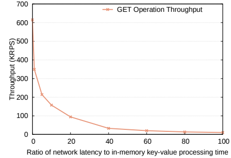
Figure 20: Throughput of memcached for relative network latencies
