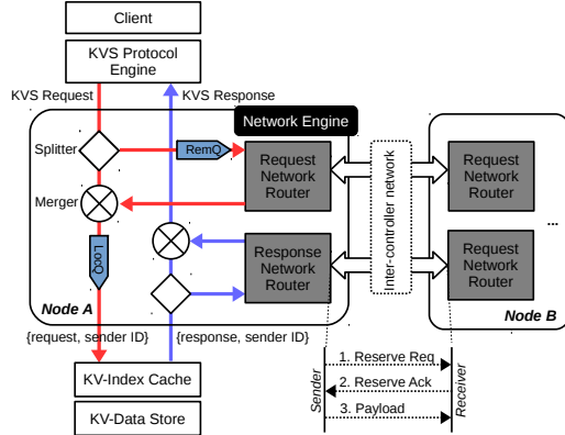
Figure 7: Network Engine Architecture
