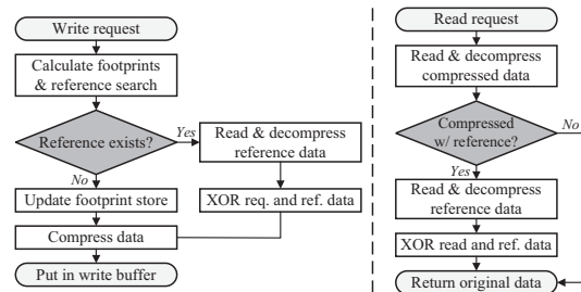
Fig. 3: Request handling procedures of DAC-FTL.
