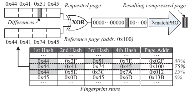
Fig. 2: The proposed dedup-assisted compression mechanism.
