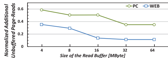
Fig. 5: Comparisons of normalized additional unbuffered page-reads for varying size of read buffer.
