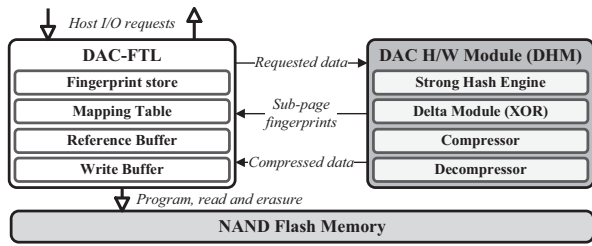
Fig. 1: An organizational overview of our target SSDs.
